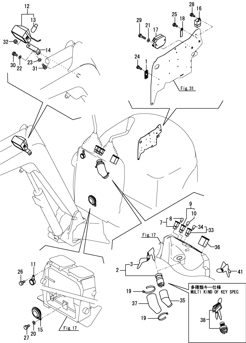
Fig.14. ELECTRIC PART(EQUIPMENT)
