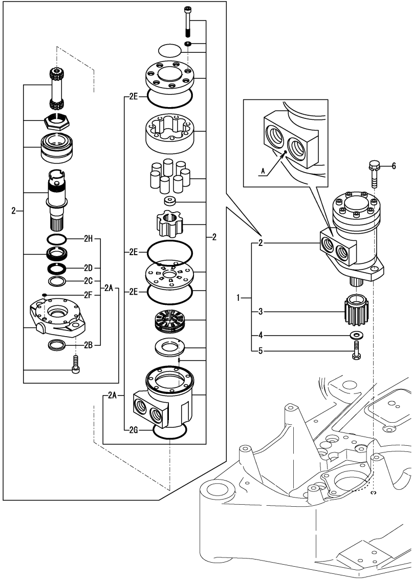
Fig.42. TURNING MOTOR(FROM M11977)
