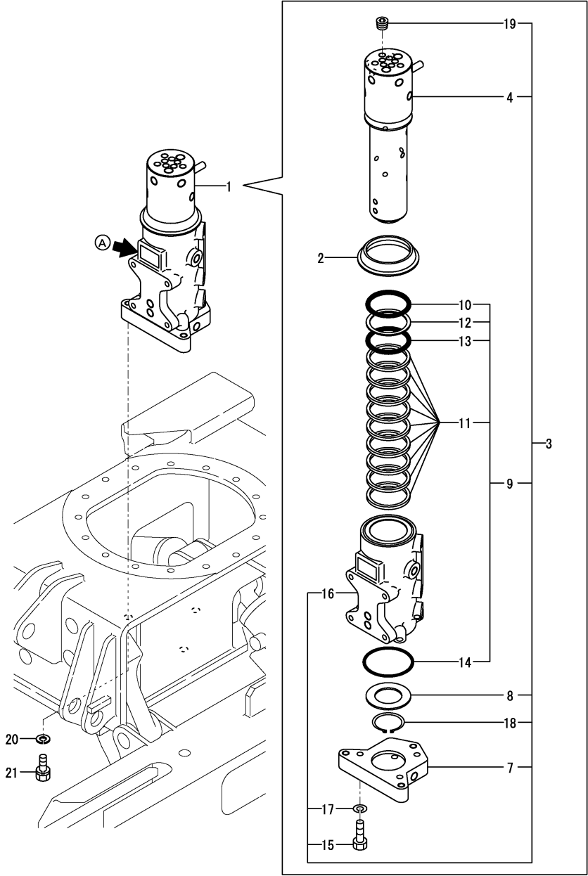
Fig.83. (44A)SWIVEL JOINT(LINK VARIABL LEG)(N SPEC.)
