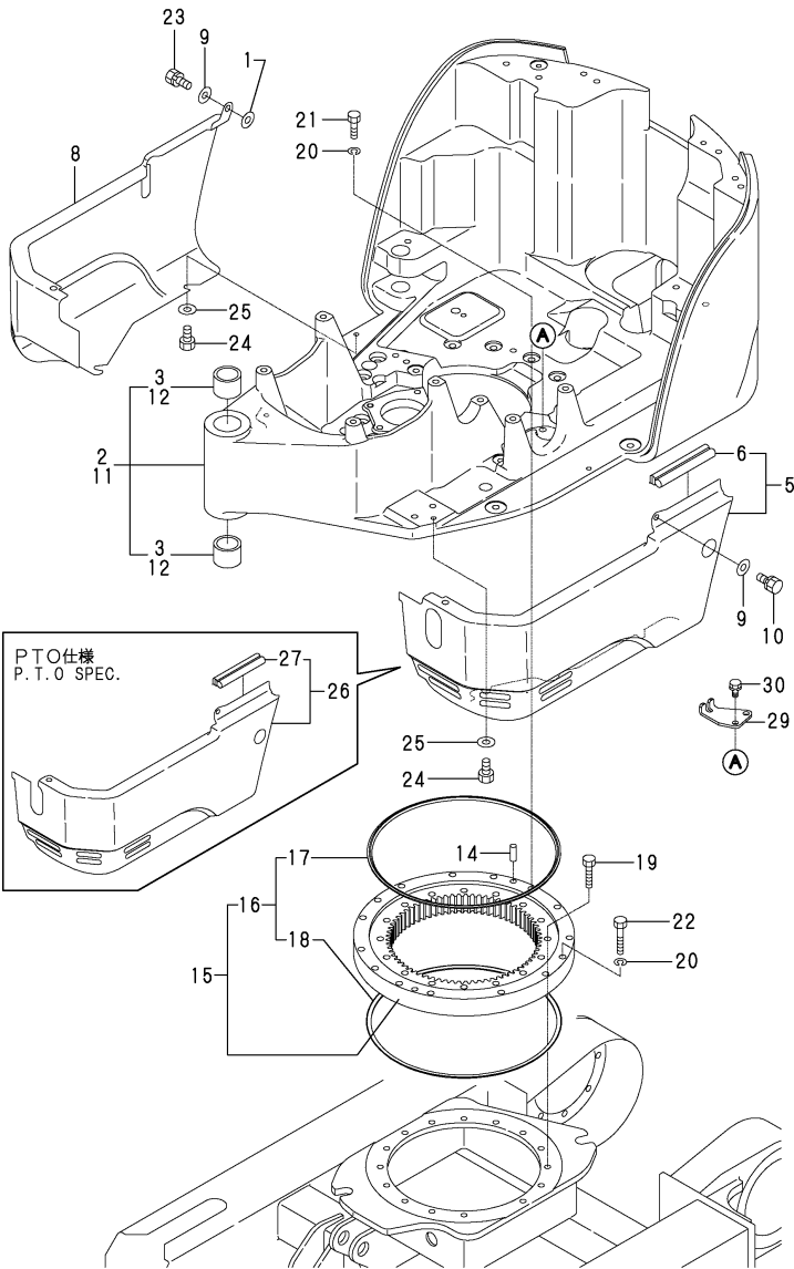
Fig.28. TURNING FRAME
