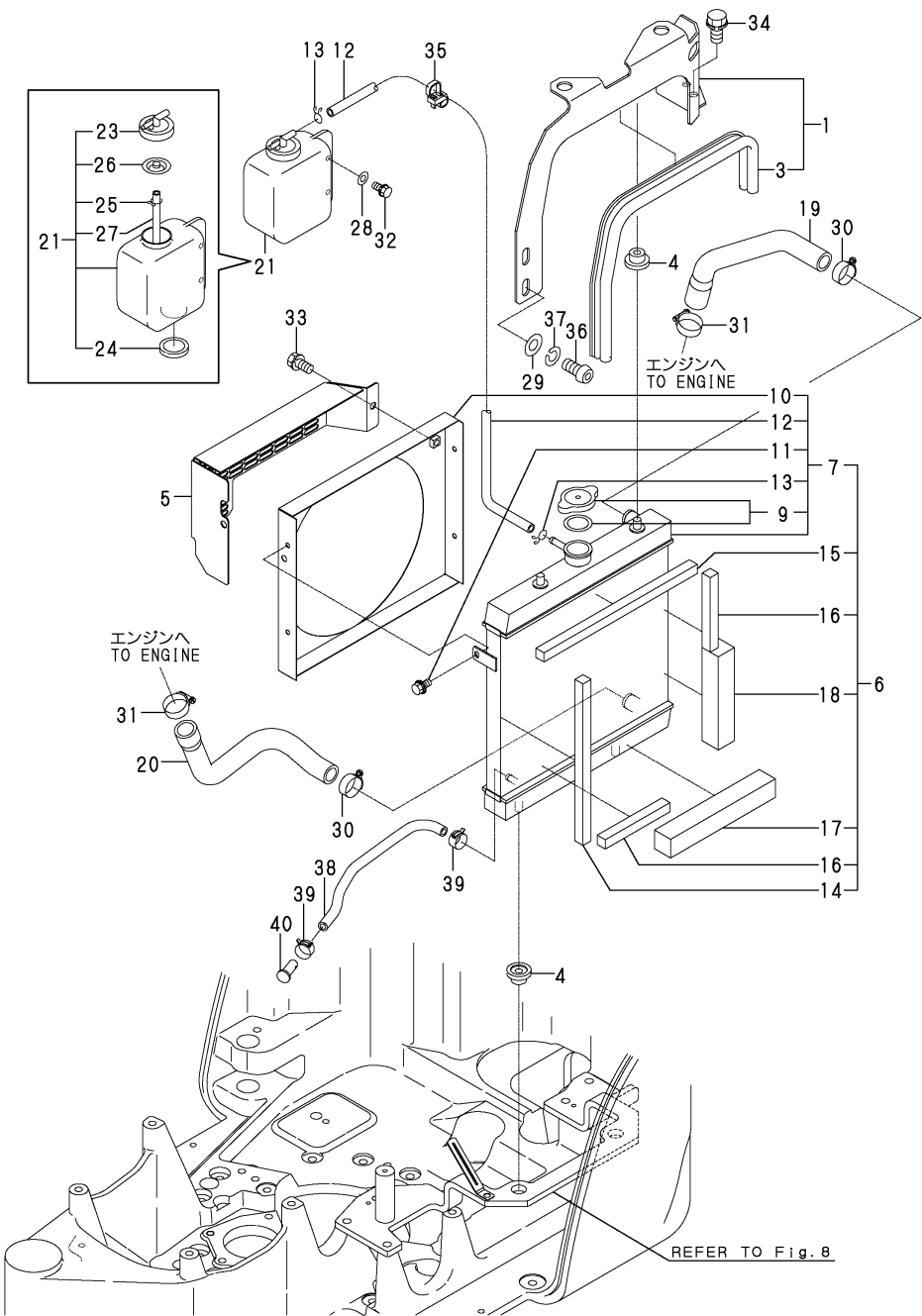
Fig.9. RADIATOR & MOUNT
